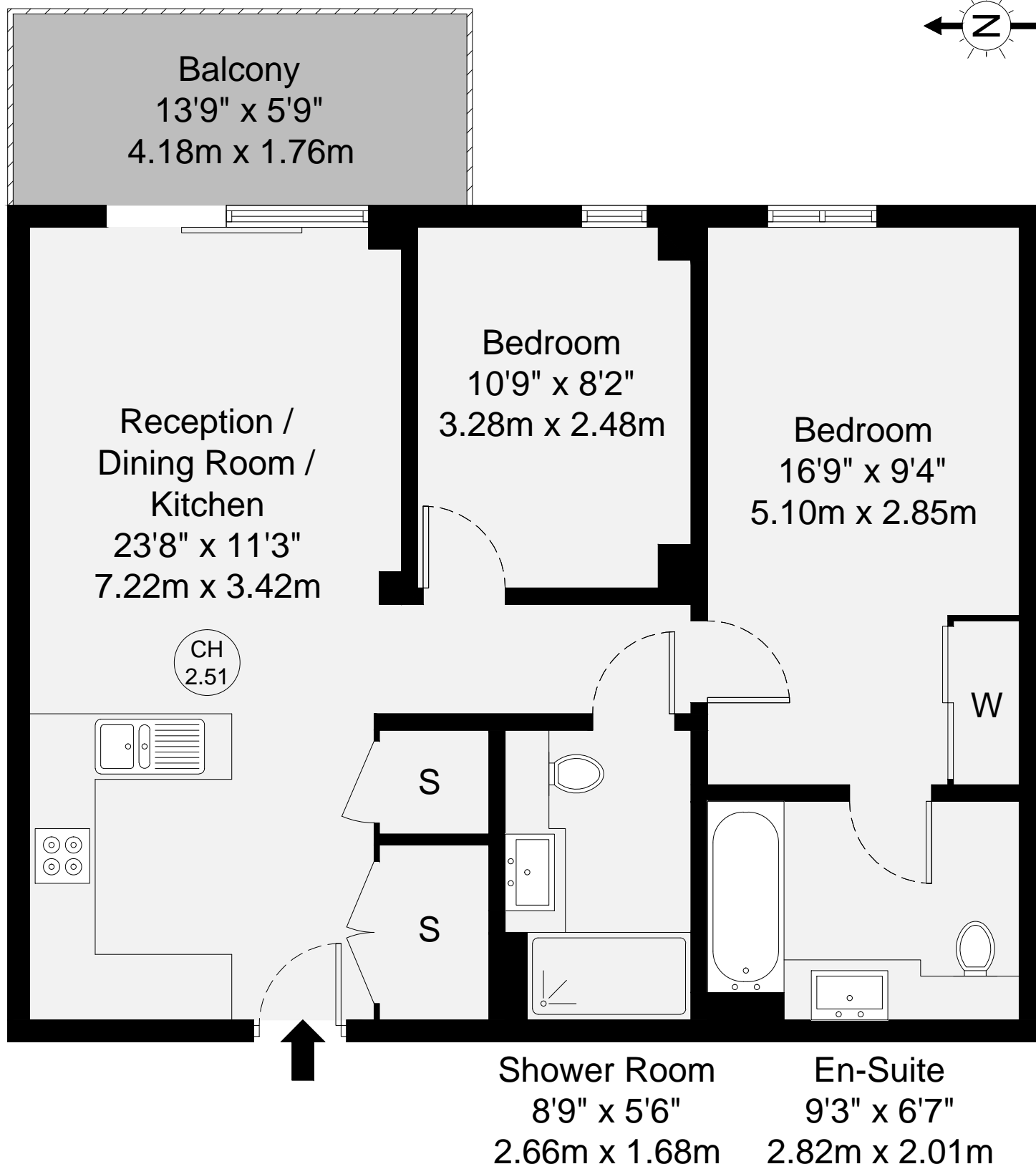
Third Floor
